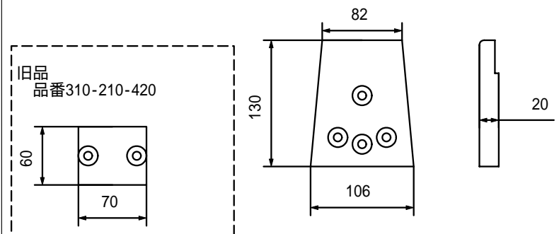
YS250/250T/303/350/350T 品番310-211-401
